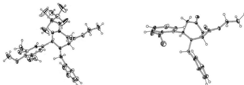
Figure 2. ORTEP drawing of crystal structures of 9 and 24 .
