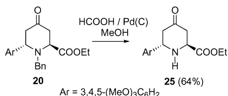
Scheme 4. Formation of 25 .
