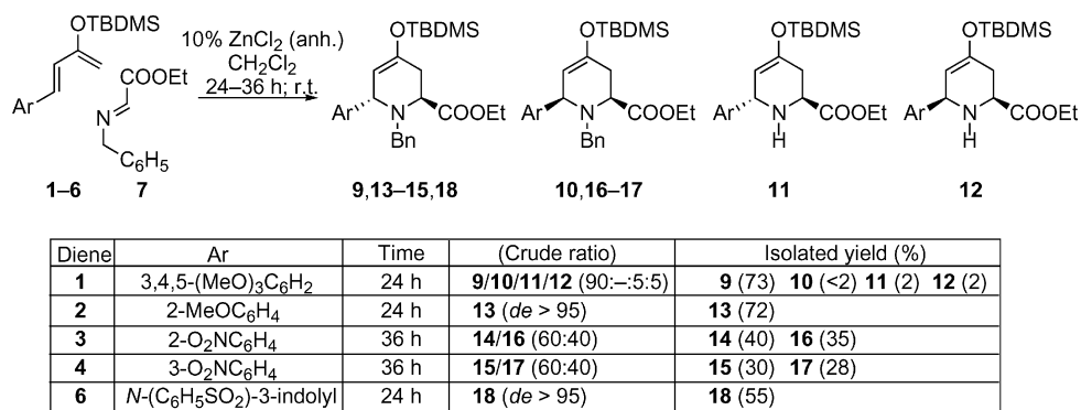
Scheme 1. Synthesis of 9–18 .
